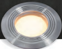
Onyx 60 R1 151D LED 1W 2.700 K - 23 lm Edelstahl 316 45 x 75 x 75 mm (HxBxT) 1 m Kabel
